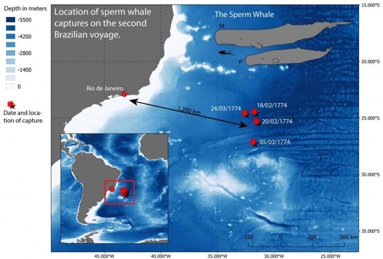
Location of sperm whale captures from the second voyage (February 5 to April 1, 1774). Nine whales were caught at four different locations, at an average depth of 5,100 meters.
